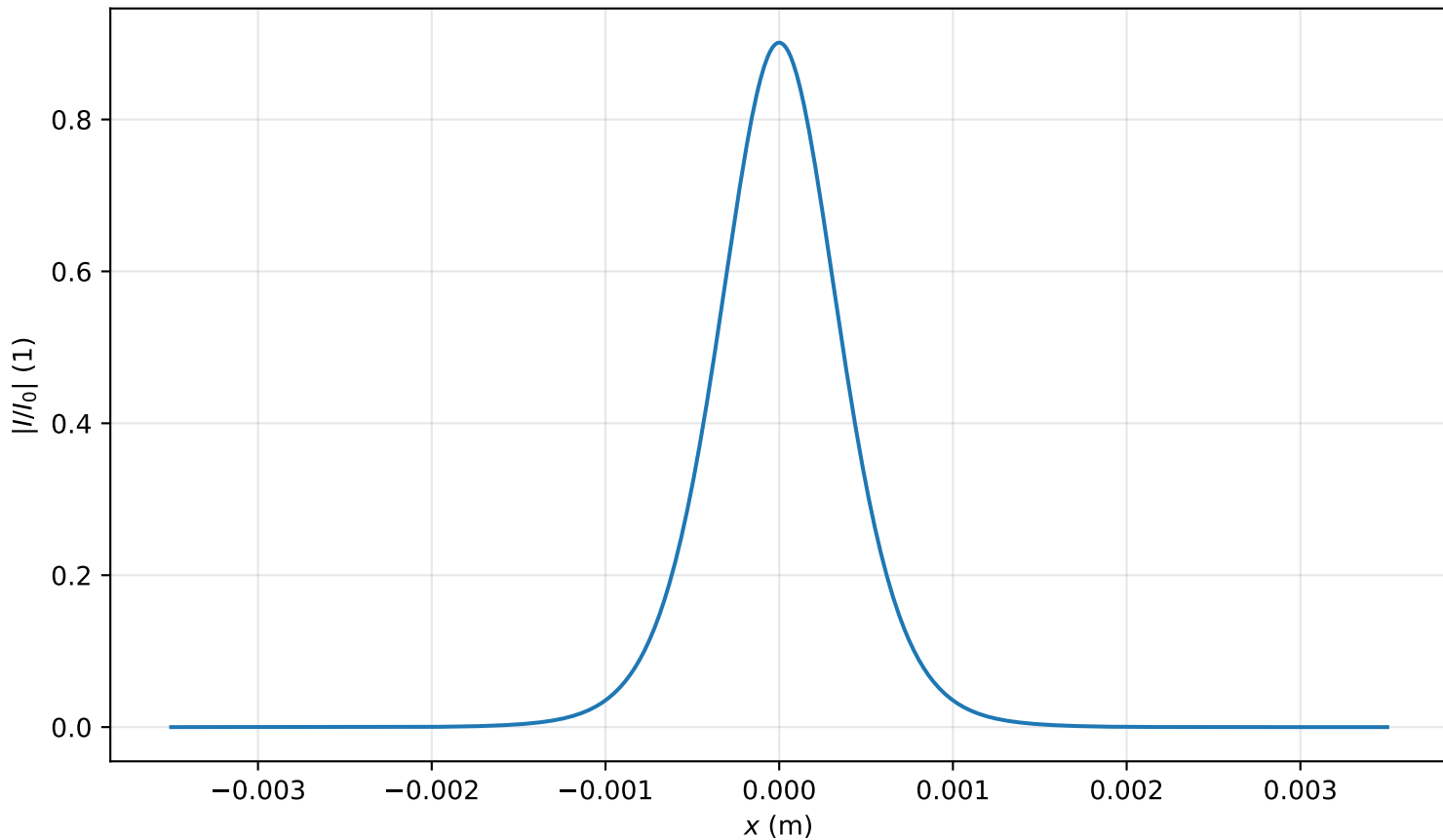
Intensity profile I(x, y = 0, z = 2.149m)/I_0 , P_{in}=0.6P_{cr} , artificial time
